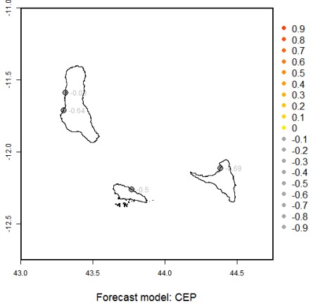
Score RPSS: RR NDJ-2020 It1
