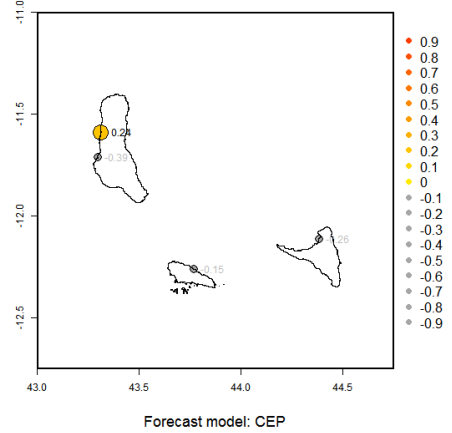
Score RPSS: RR DJF-2020 It1
