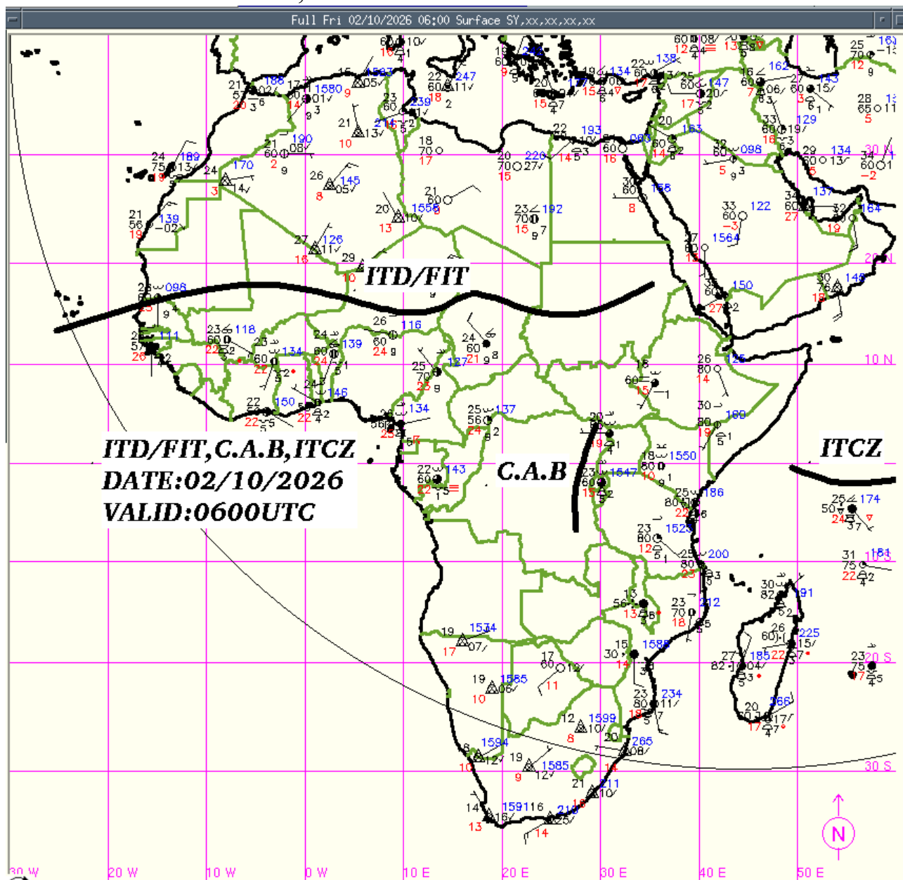
Tabulated positions of the ITD: 2 nd October 2026
