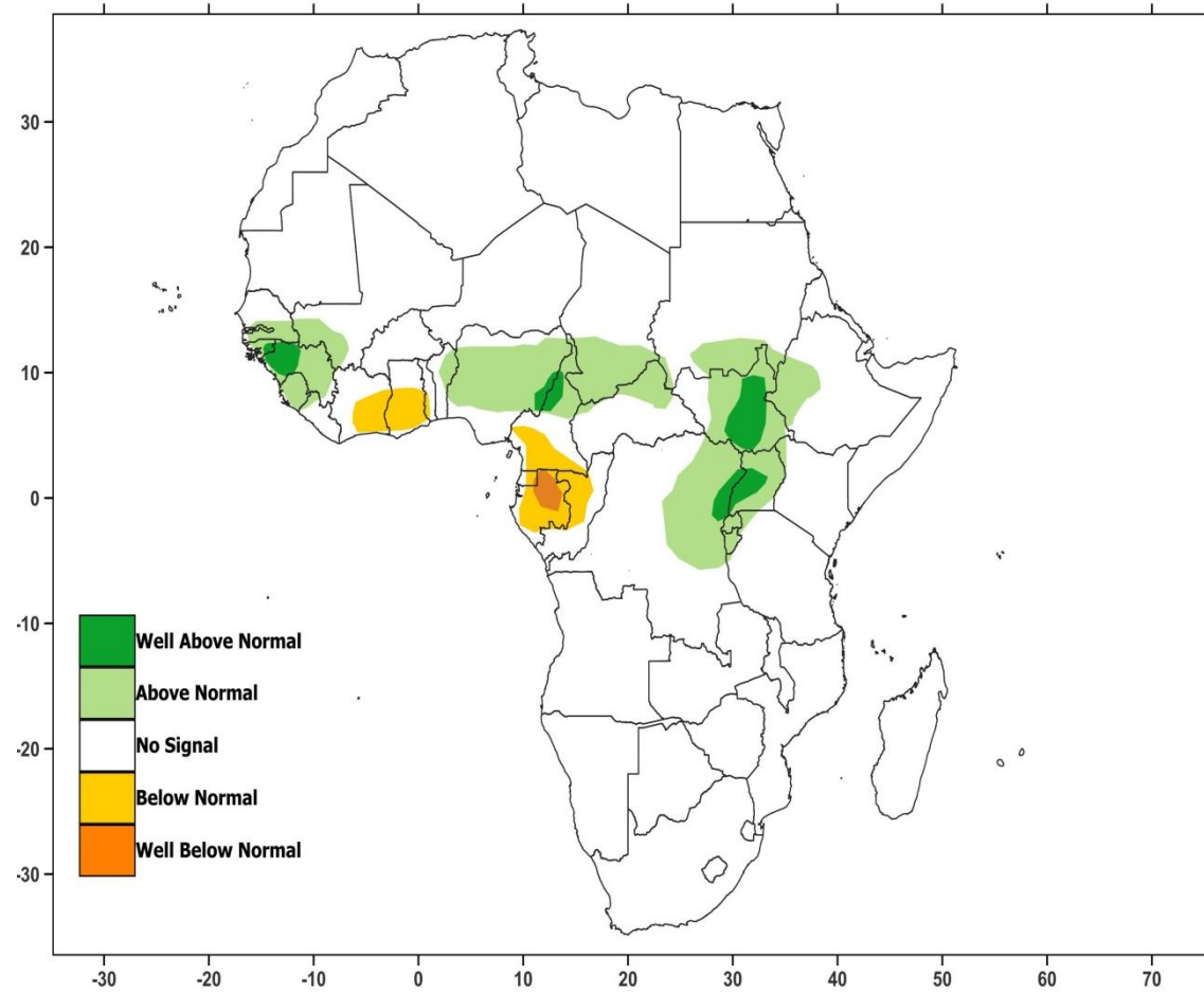
PRCIP FCST WEEK1 14-20 SEPTEMBER 2022
