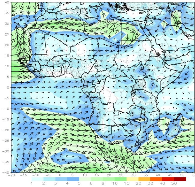
GFS 700mb week1 Mean Divergence Anomaly ( 10 \times 10^{-5} / s ) Period: 18z22Sep2022 - 18z28Sep2022
