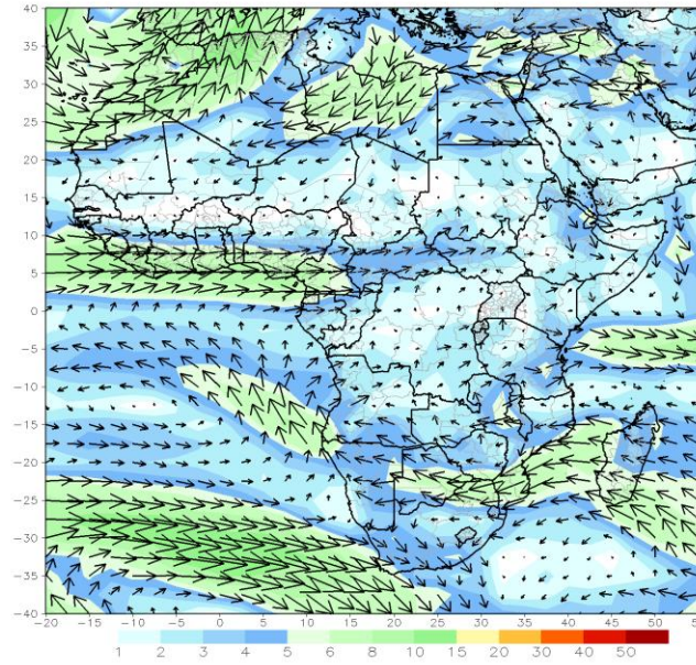
GFS 700mb week2 Mean Divergence Anomaly ( 10 \times 10^{-5}/s ) Period: 18z29Sep2022 – 18z05Oct2022
