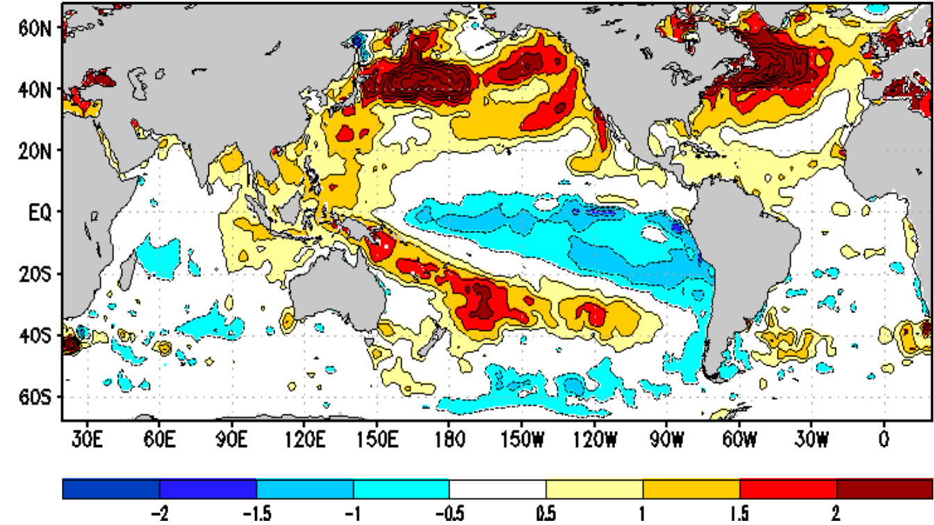
SST Anom. for the Week From 21Aug2022 to 17Sep2022
