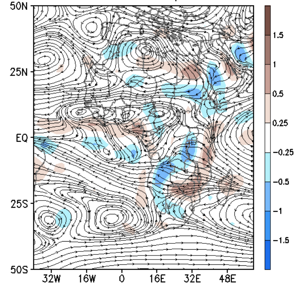
CDAS 850hPa Divergence and Wind Tot. Dekad: 11–20 Sep 2022
