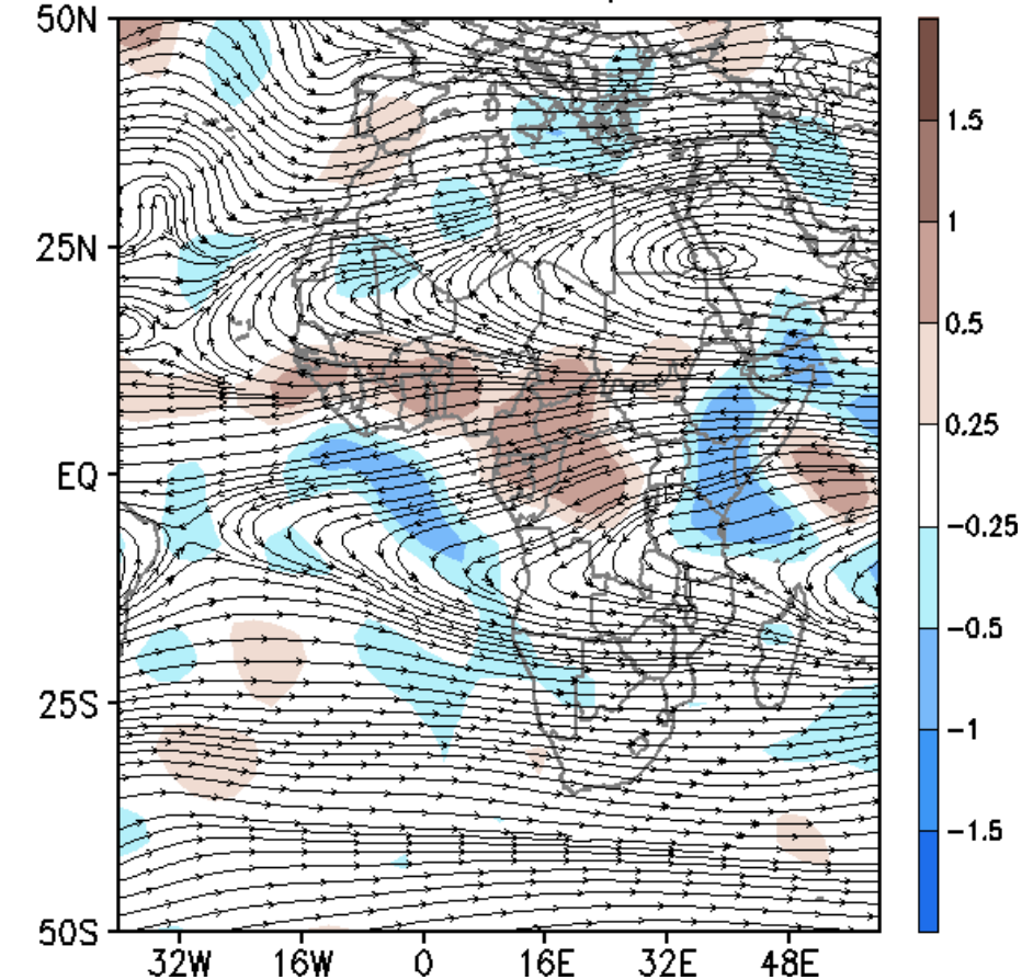
CDAS 200hPa Divergence and Wind Tot. Dekad: 11–20 Sep 2022
