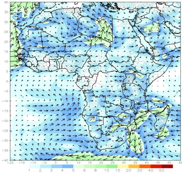
GFS 850mb week1 Mean Divergence Anomaly ( 10 \times 10^{-5} / s ) Period: 18z22Sep2022 - 18z28Sep2022
