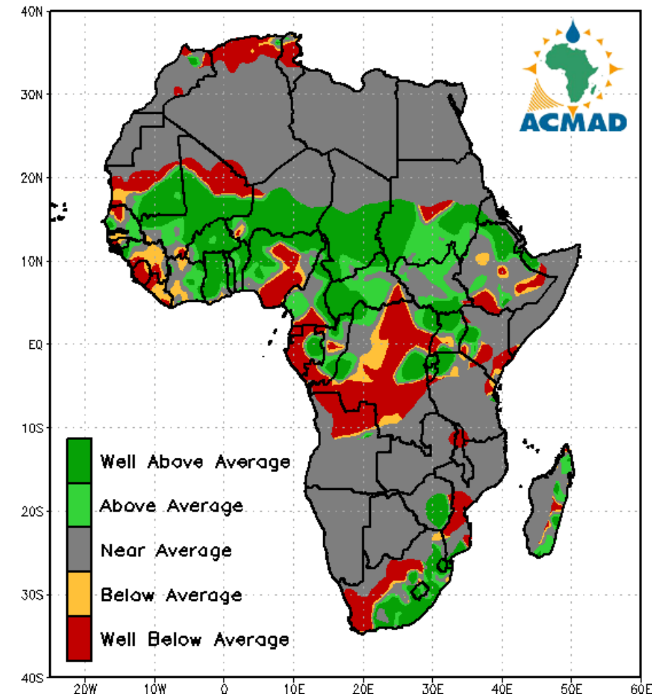
CPC-Uni 7day Precipitation in Percent of Average (%) Period: 14Sep2022 to 20Sep2022
