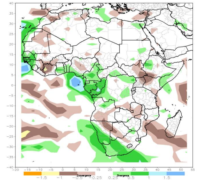
GFS 200mb week1 Mean Divergence Anomaly ( 10 \times 10^{-5} / s ) Period: 18z22Sep2022 - 18z28Sep2022
