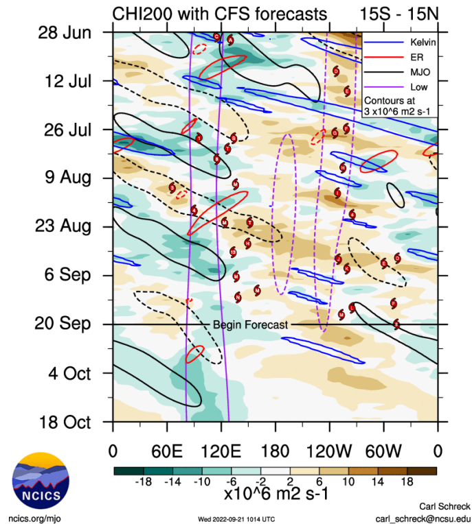
Average Anomalies in the band 15S-15N
