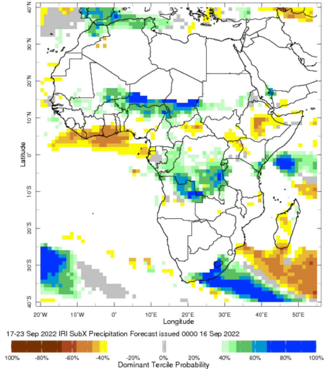
Figure 37: Precipitation and Anomaly forecast
