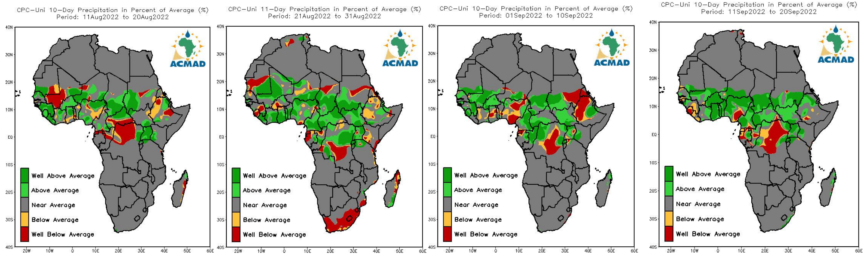
Figure 2: This maps display decadal average precipitation in percent of average
