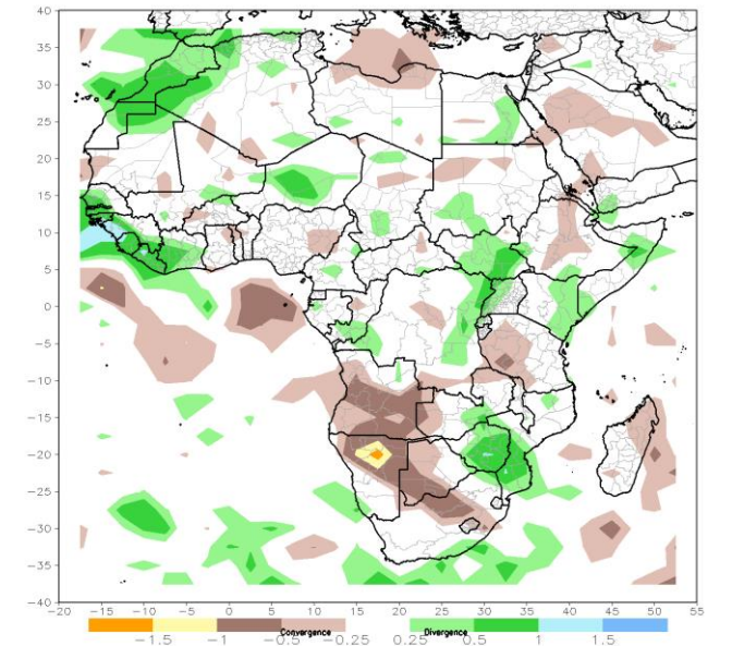
GFS 200mb week2 Mean Divergence Anomaly ( 10 \times 10^{-5}/s ) Period: 18z29Sep2022 – 18z05Oct2022
