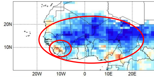
Fcst_nmme_sst_Avr-lc_CHIRPS_JJA-2024
