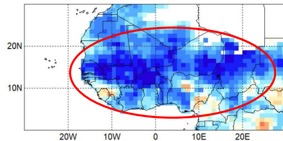
Fcst_nmme_sst_Avr-lc_CHIRPS_JAS-2024
