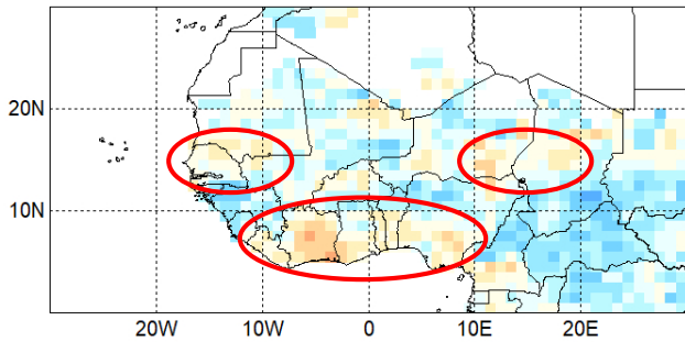
Skill_nmme_sst_Avr-lc_CHIRPS_MJJ-2024
