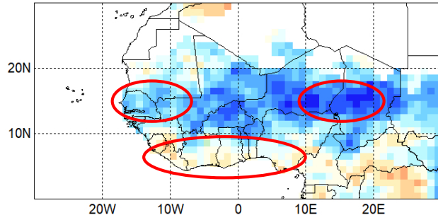
Fcst_nmme_sst_Avr-lc_CHIRPS_MJJ-2024
