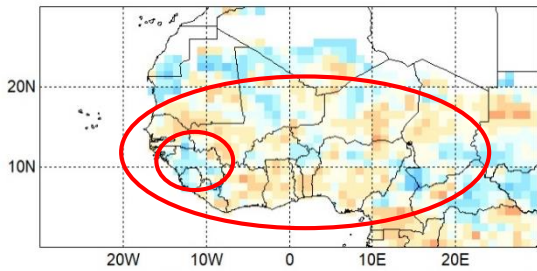
Skill_nmme_sst_Avr-lc_CHIRPS_JJA-2024
