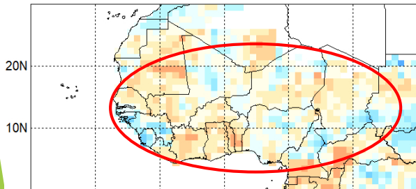
Skill_nmme_sst_Avr-lc_CHIRPS_JAS-2024
