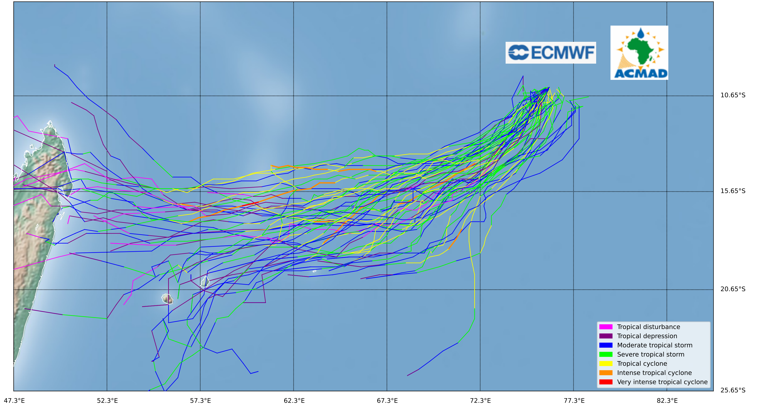
Tropical Cyclone forecast, valid from 12UTC on 14 to 24 Nov 2024 TC name: BHEKI (source: ECMWF ensemble model)
