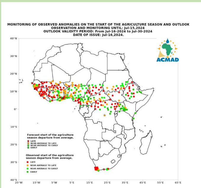
Characteristic of the Onset of the Agricultural Season over Africa (16-30 July 2024)
