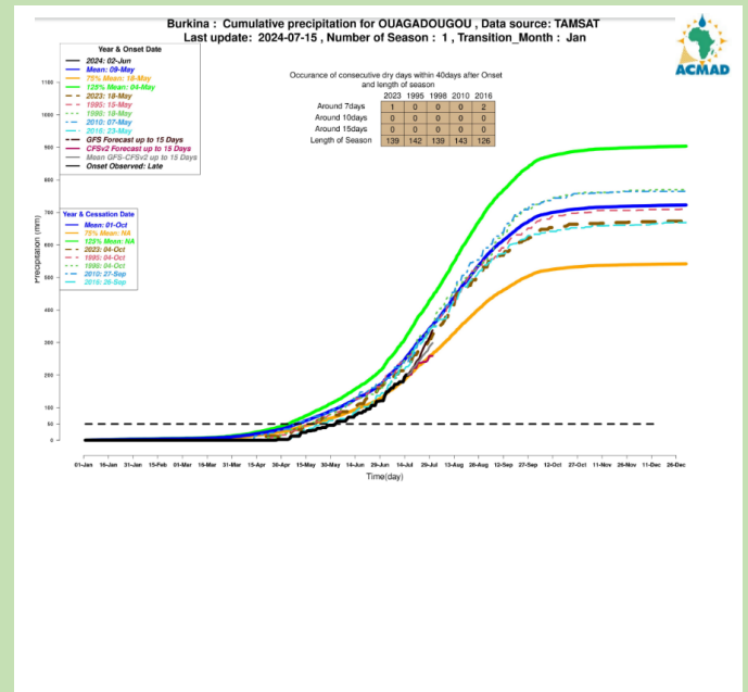
Cumulative Precipitation Profile in Ouagadougou, Burkina Faso
